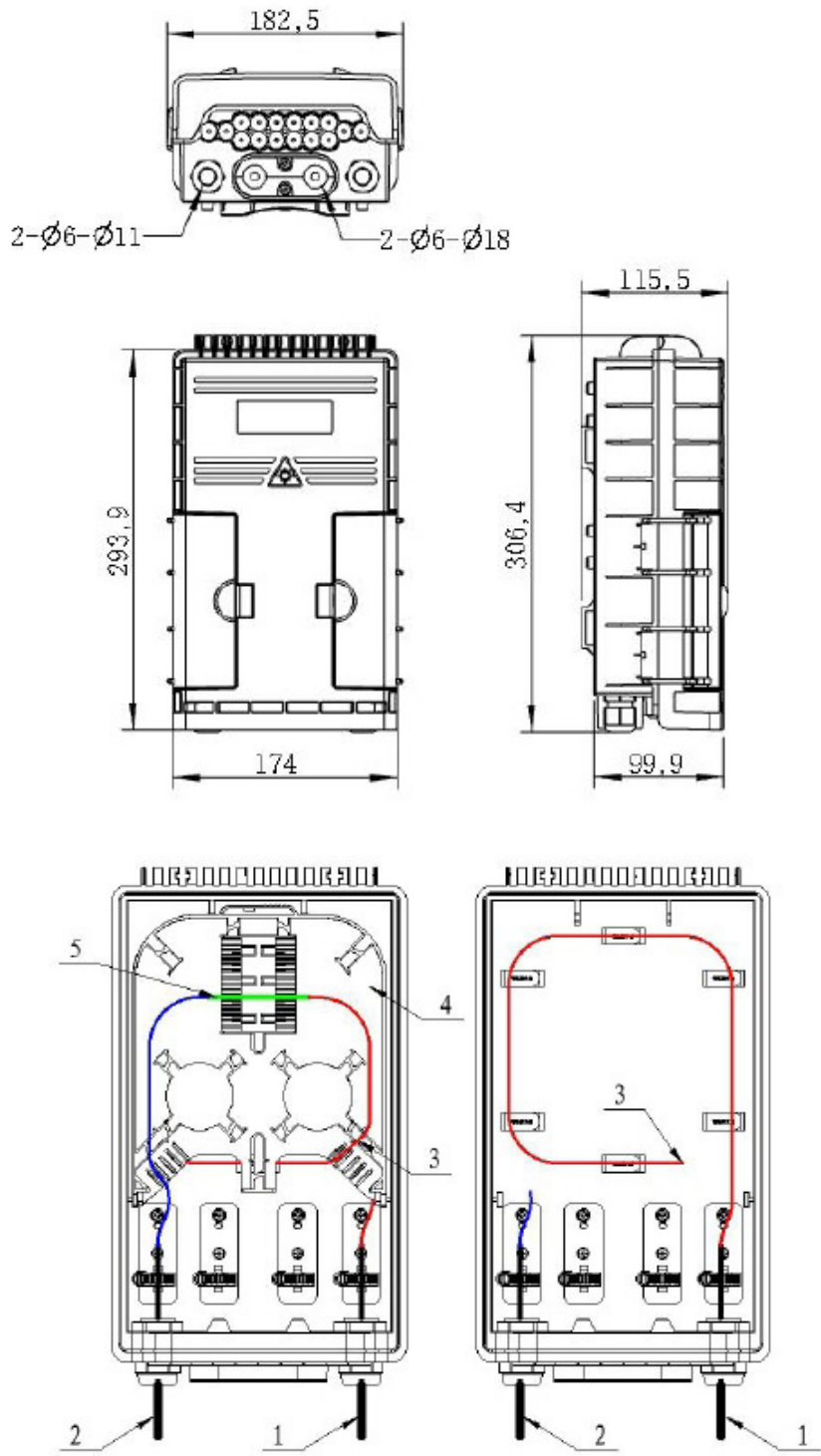
1 - Cable entry port 2 - Cable output port 3 - Fiber optic cable 4 - Fiber optic splice tray 5 - Heat protection shrinkable sleeve
