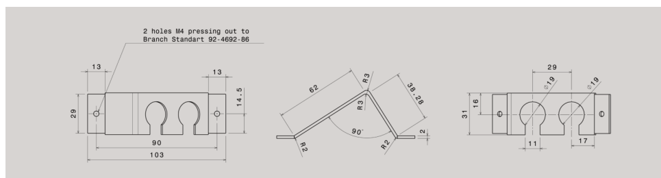
Cable entry plate rechargeable angular
