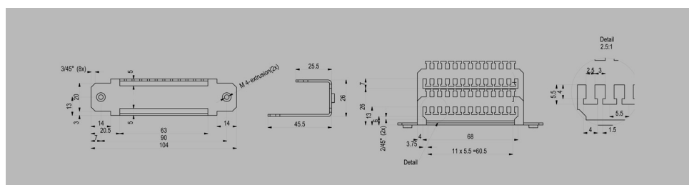
Cable entry plate rechargeable, straight, 24/48:
